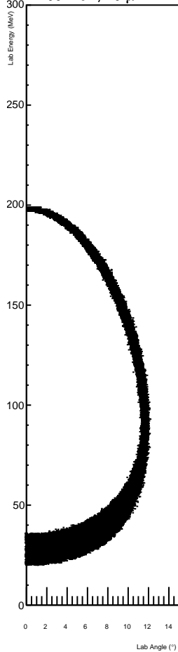
295 MeV, 10 \mu\text{m} Al
