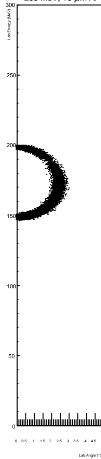
295 MeV, 10 \mu\text{m} Al
