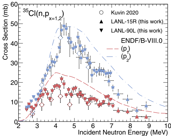
FIG. 5. Summary of newest data from WNR for ^{35}\text{Cl}(n, p_x) partial cross sections to ^{35}\text{S} excited states. Though not shown, data for x = 3, 4 , and 5 were also collected and will be available in EXFOR.
