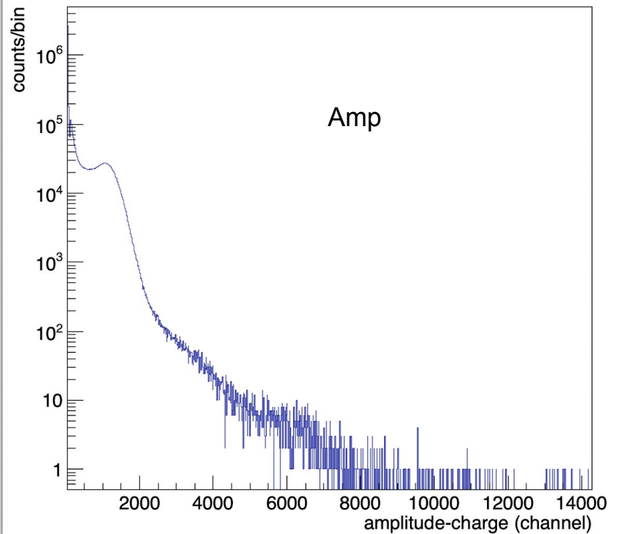
cal2-Cs137_A_u1_C6D6_run107774
