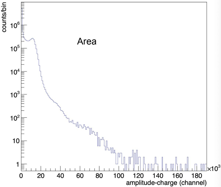
cal2-Cs137_A_u1_C6D6_run107774
