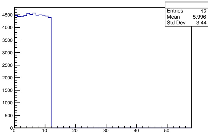
SILI/PKUP ratio
