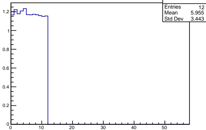
Normalised resonance integral
