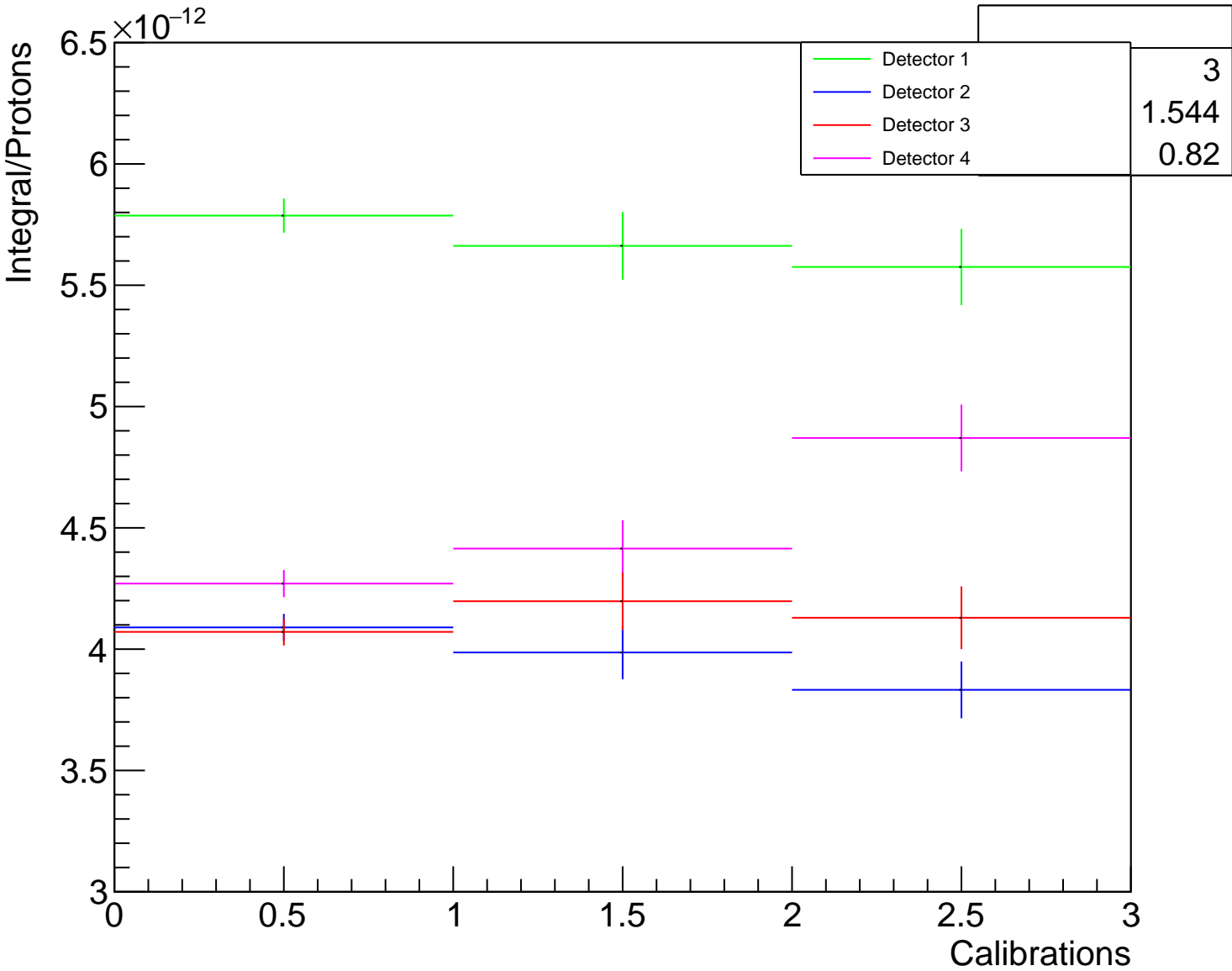
Resonance 3: Integral/Protons Vs Cut for All Detectors
