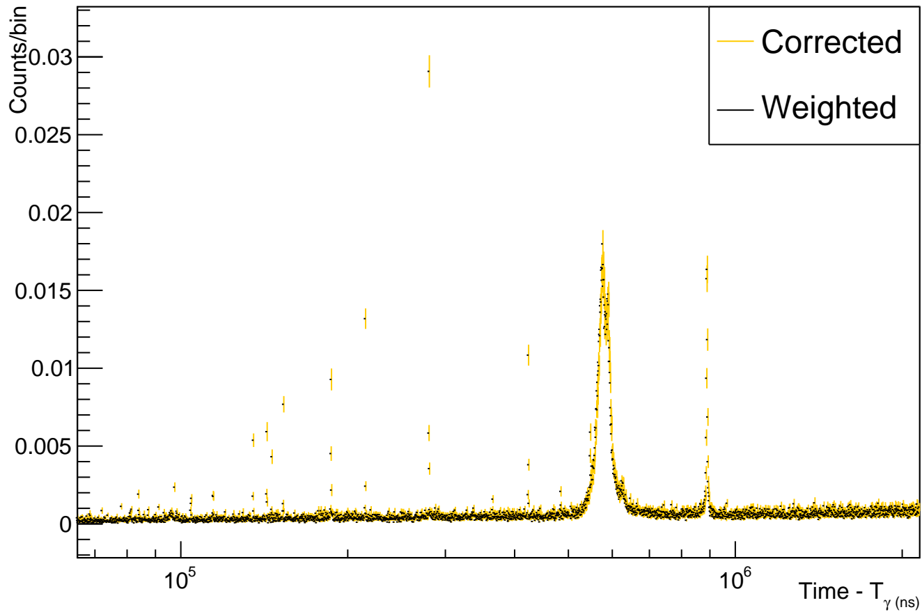
Deadtime*Weighted Spectra Vs Weighted Spectra: Parasitic Det3
