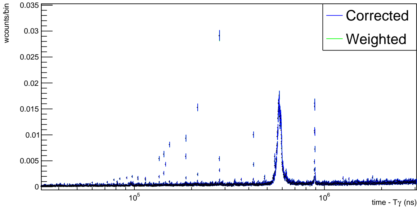
Deadtime*Weighted Spectra Vs Weighted Spectra: Parasitic Det2
