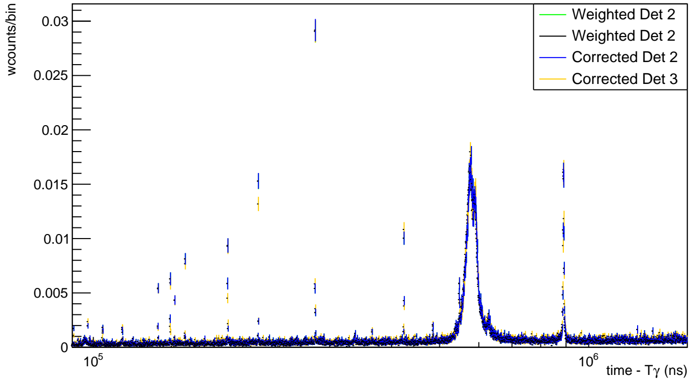
Deadtime*Weighted Spectra Vs Weighted Spectra: Parasitic All Dets
