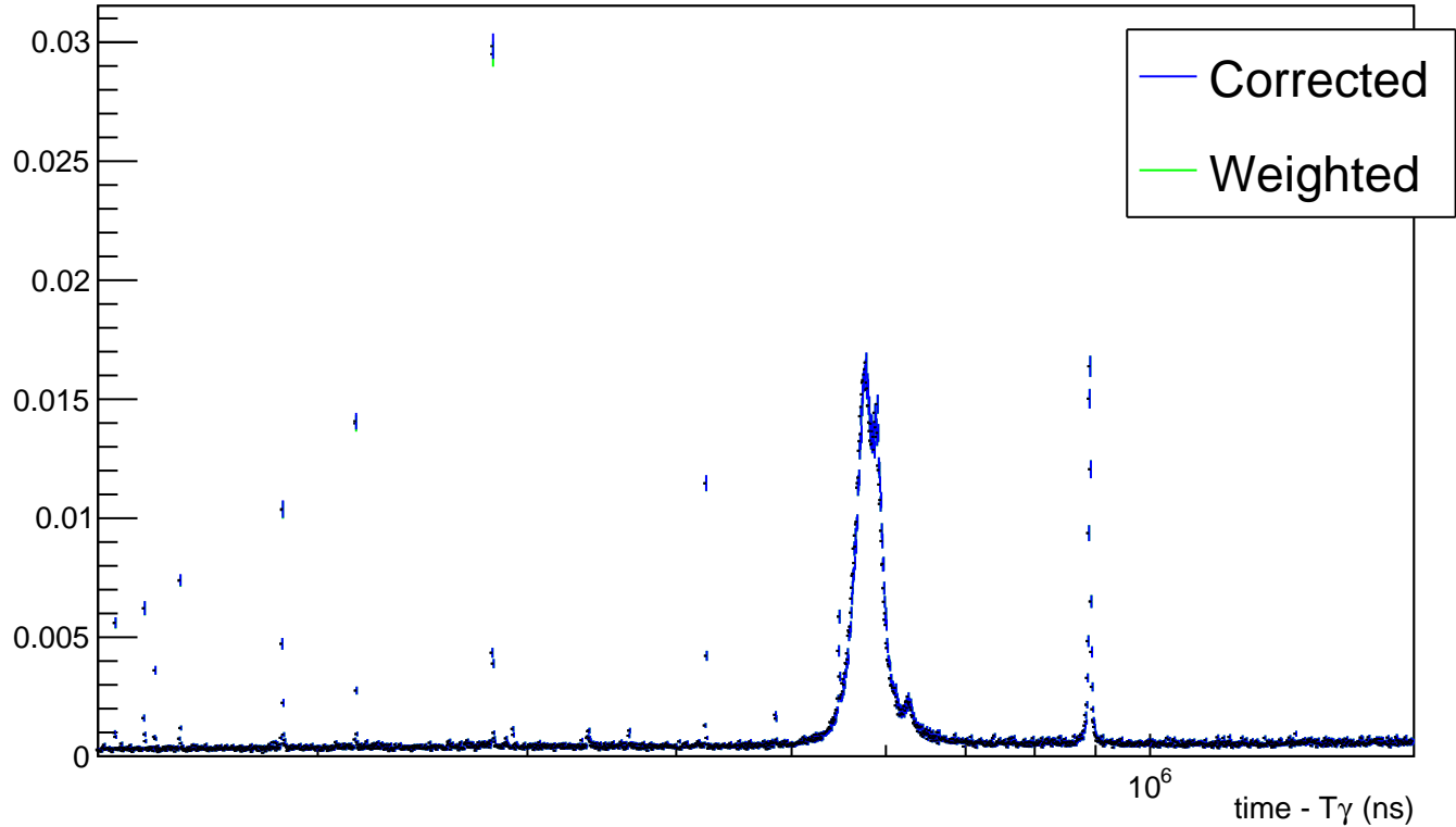
Deadtime*Weighted Spectra Vs Weighted Spectra: Dedicated Det2
