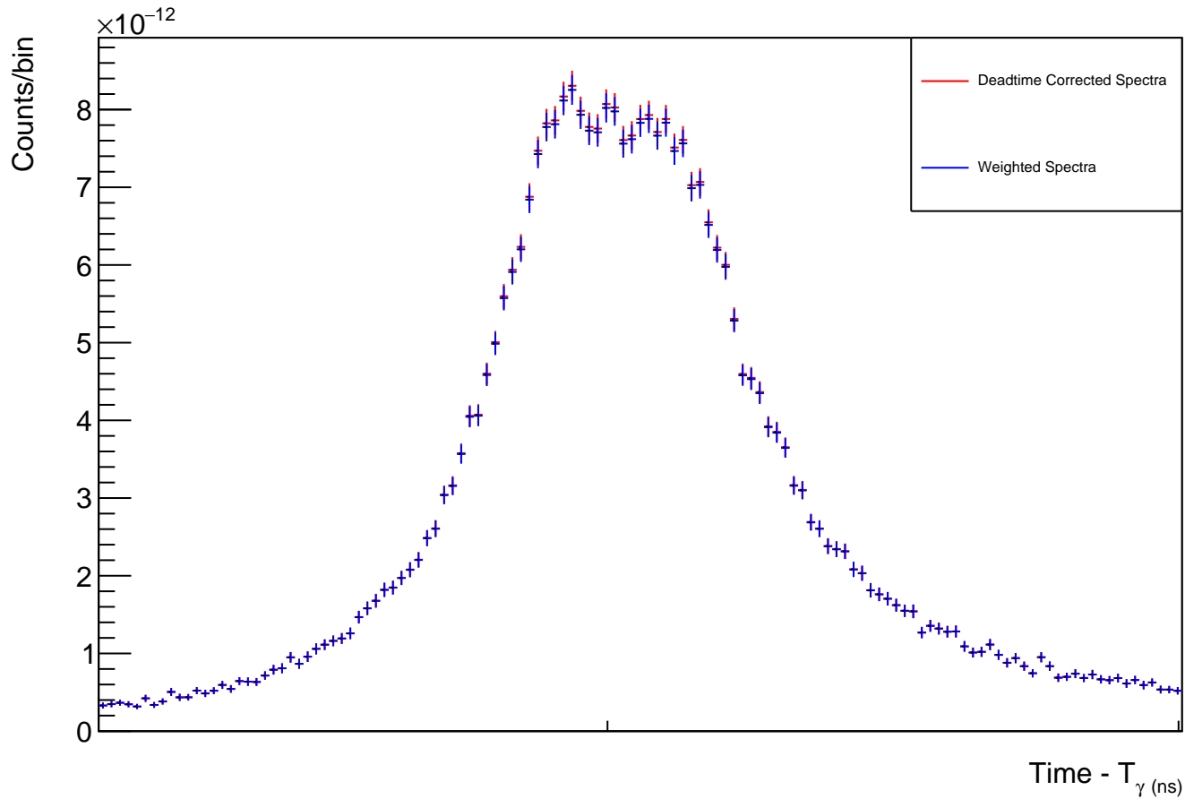
Deadtime Corrected Spectra Vs Weighted Spectra Detector 3: Dedicated
