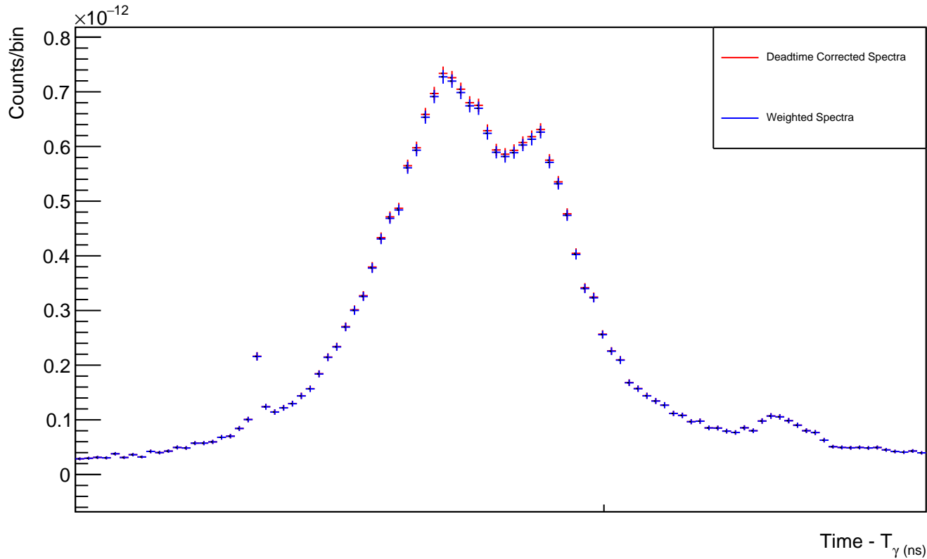
Deadtime Corrected Spectra Vs Weighted Spectra Detector 1: Dedicated
