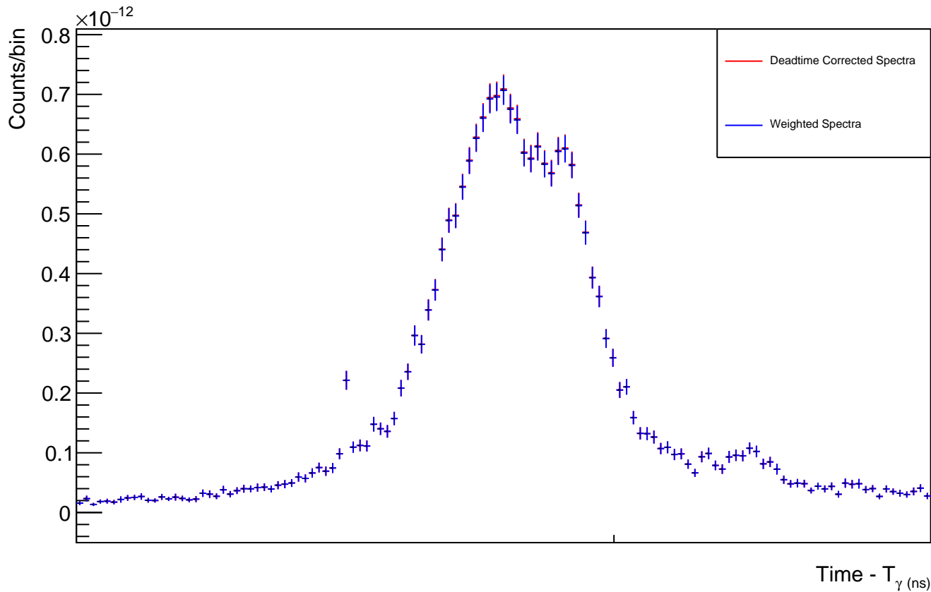
Deadtime Corrected Spectra Vs Weighted Spectra Detector 1: Parasitic
