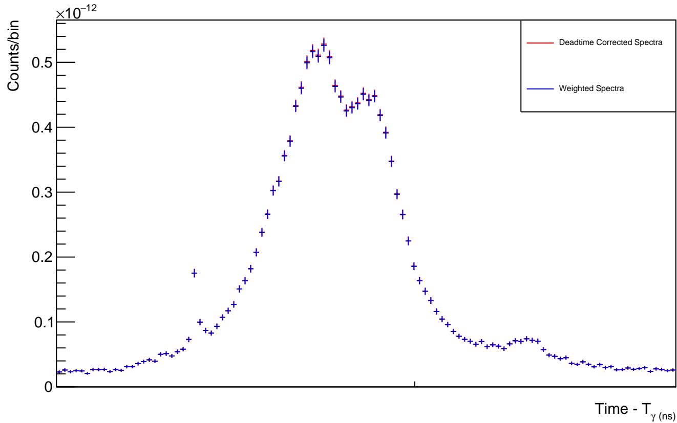
Deadtime Corrected Spectra Vs Weighted Spectra Detector 3: Dedicated
